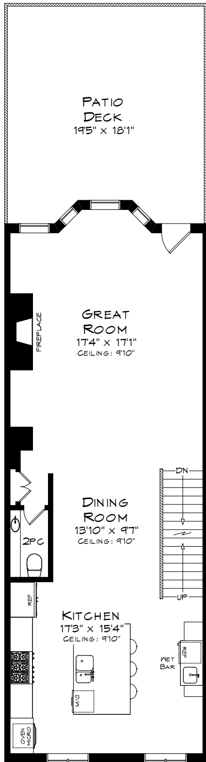
SECOND LEVEL 893 SQUARE FEET
