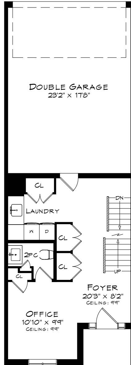
GROUND LEVEL 452 SQUARE FEET + 438 SF (GARAGE)
